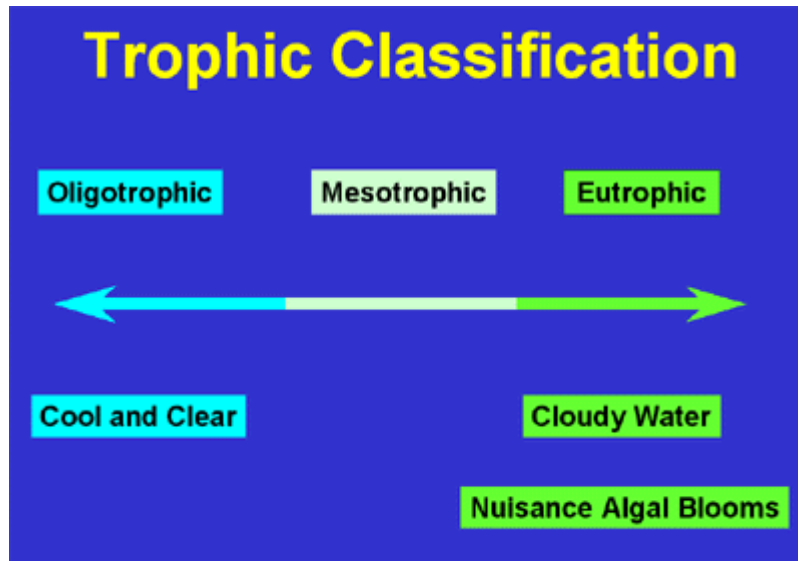
Figure G-3: Trophic Phases
