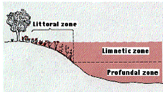
Figure G-1: Lake zones
