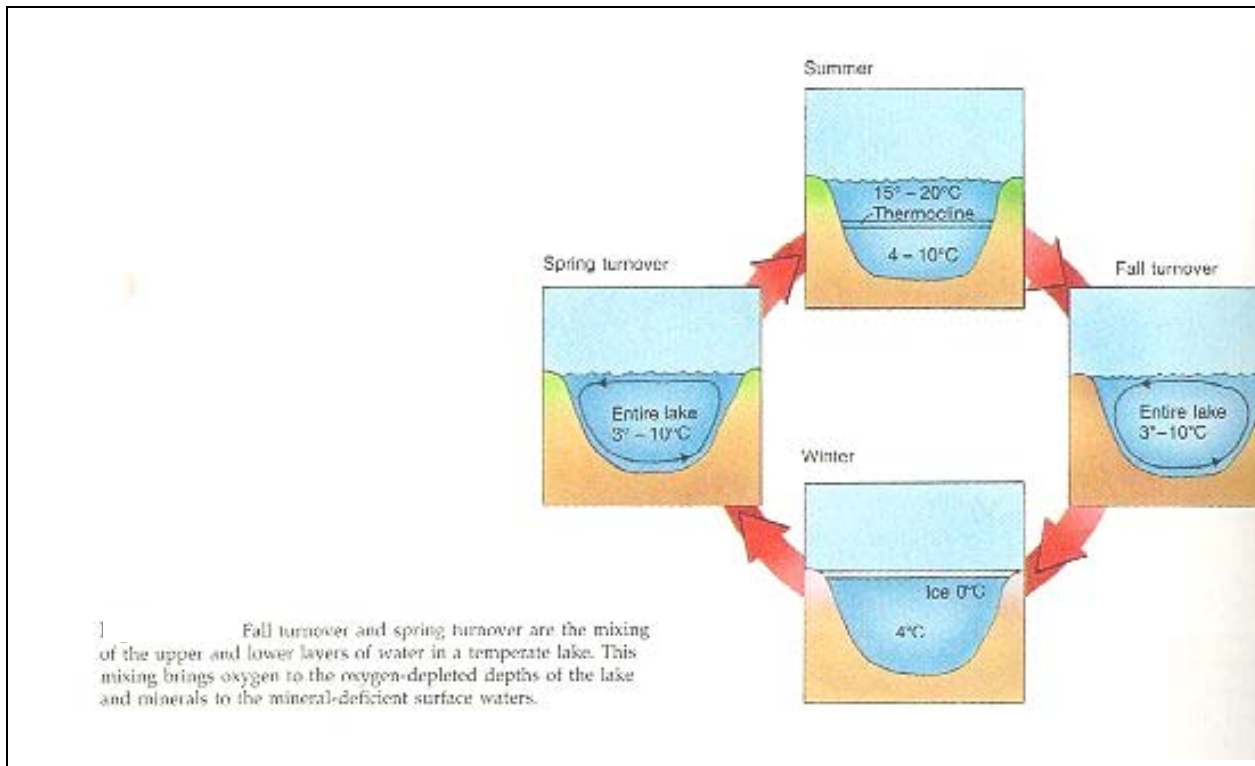
Figure G-2: Lake Temperature Seasonal Change
