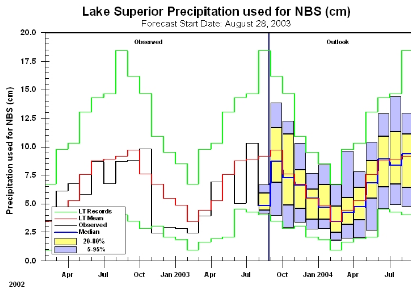
Figure E-3 - NOAA Probabilistic Precipitation Outlook
