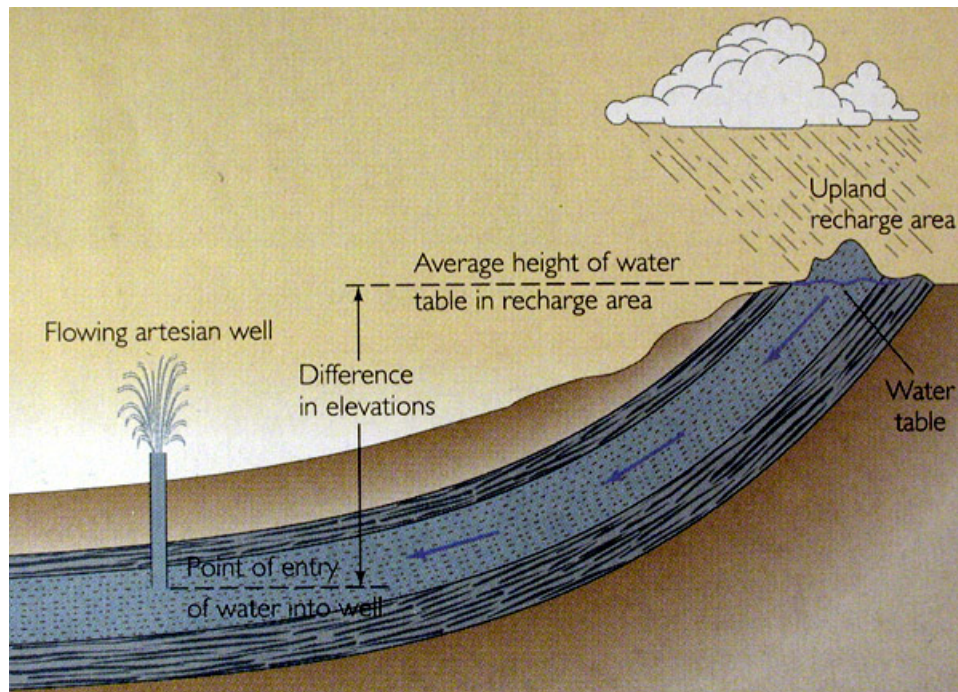
Figure B-3: Upland recharge area for a confined aquifer. (Press and Siever, 1998)
