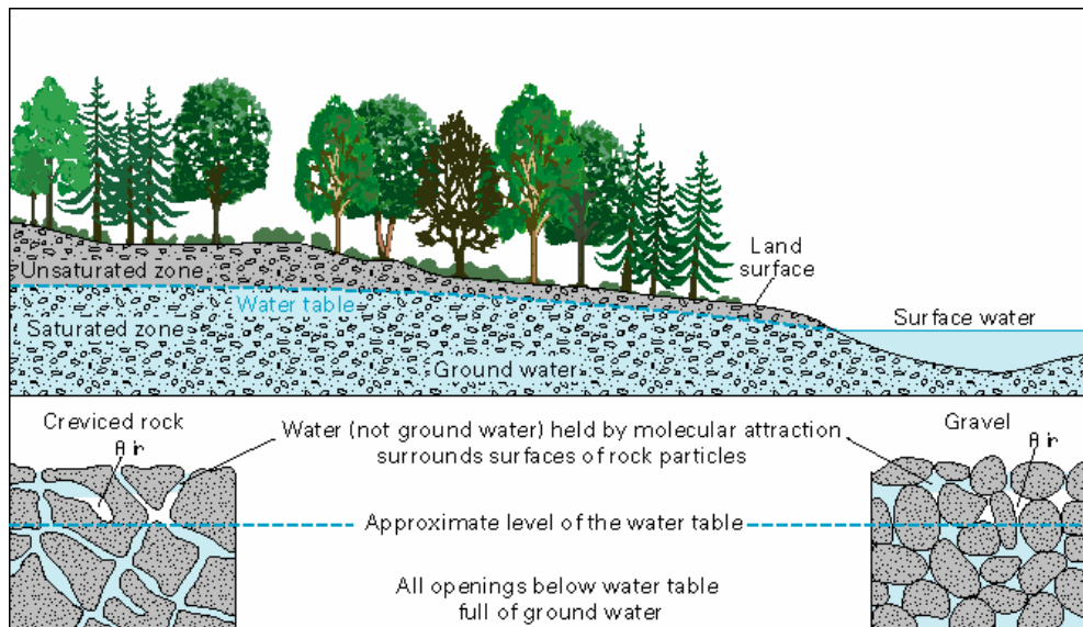
Figure B-2: How groundwater occurs in rocks. (U.S. Geological Survey)
