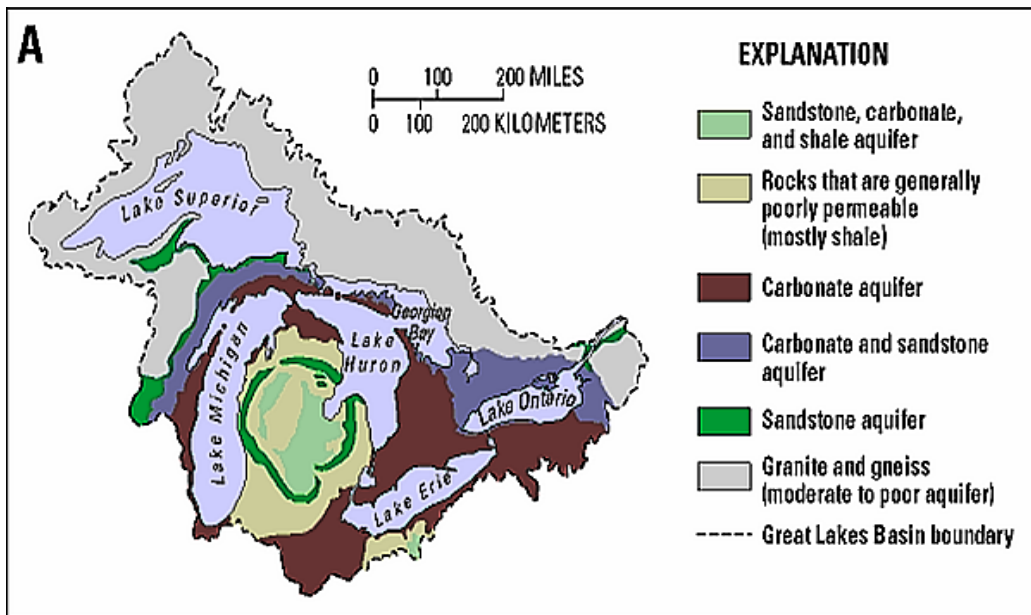
Figure B-1: Bedrock aquifers of the Great Lakes - St. Lawrence River basin (modified from Great Lakes Commission, 1975)
