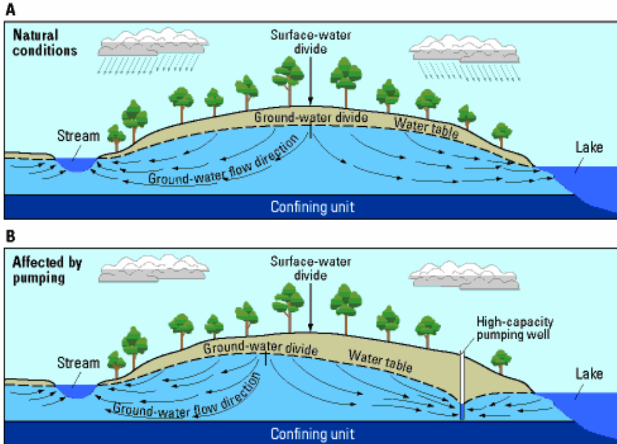
Figure B-4: Generalized groundwater flow (A) under natural conditions and (B) affected by pumping. In figure B, water flows from the lake into the groundwater system when affected by high-capacity pumping. (U.S. Geological Survey)
