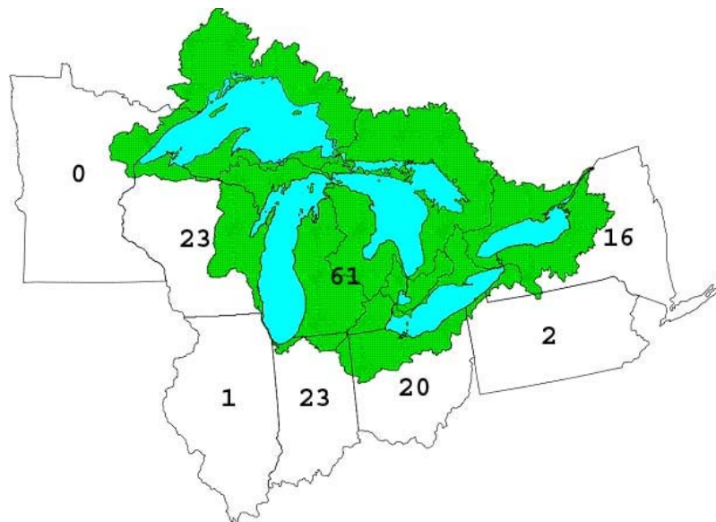
Figure B-5: Number of U.S. Geological Survey groundwater observation wells within or adjacent to the Great Lakes - St. Lawrence River basin for which water levels are monitored. (U.S. Geological Survey)
