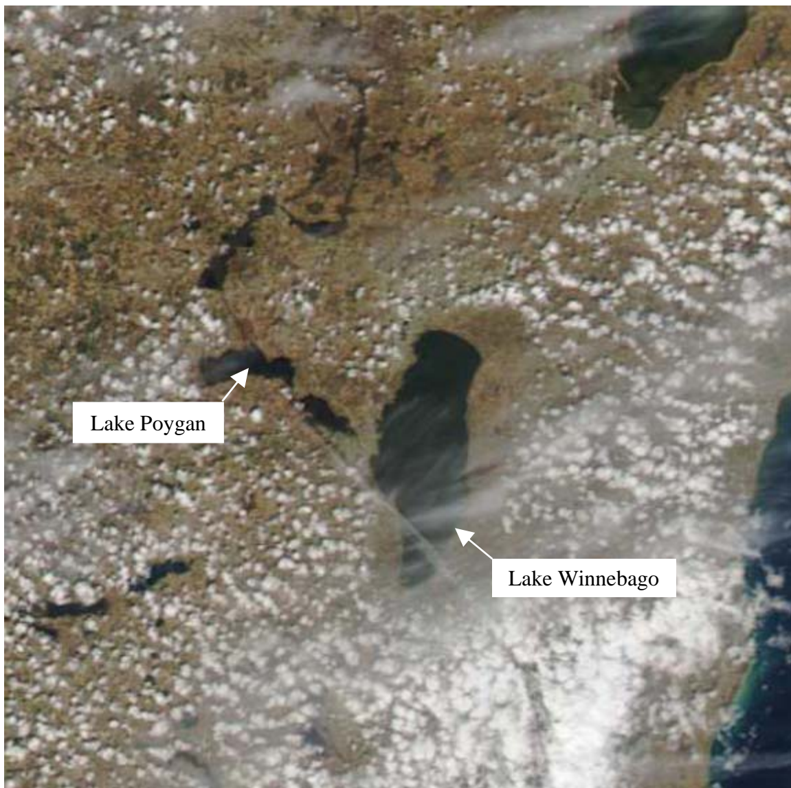
Satellite image taken April 24, 2011 (NOAA CoastWatch - Great Lake Region)
